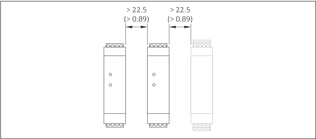
23 Minimum distance between additional Safety Barrier Promass 100 or other modules.Engineering unit mm (in)
