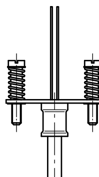
Measuring insert prepared for transmitter mounting
